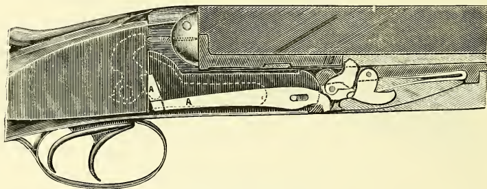
Trulock's Ejecting Mechanism.
